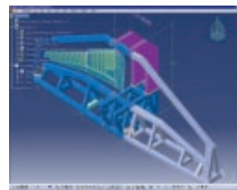
CATIA – Equipment Support Structures 2 (ESS)
